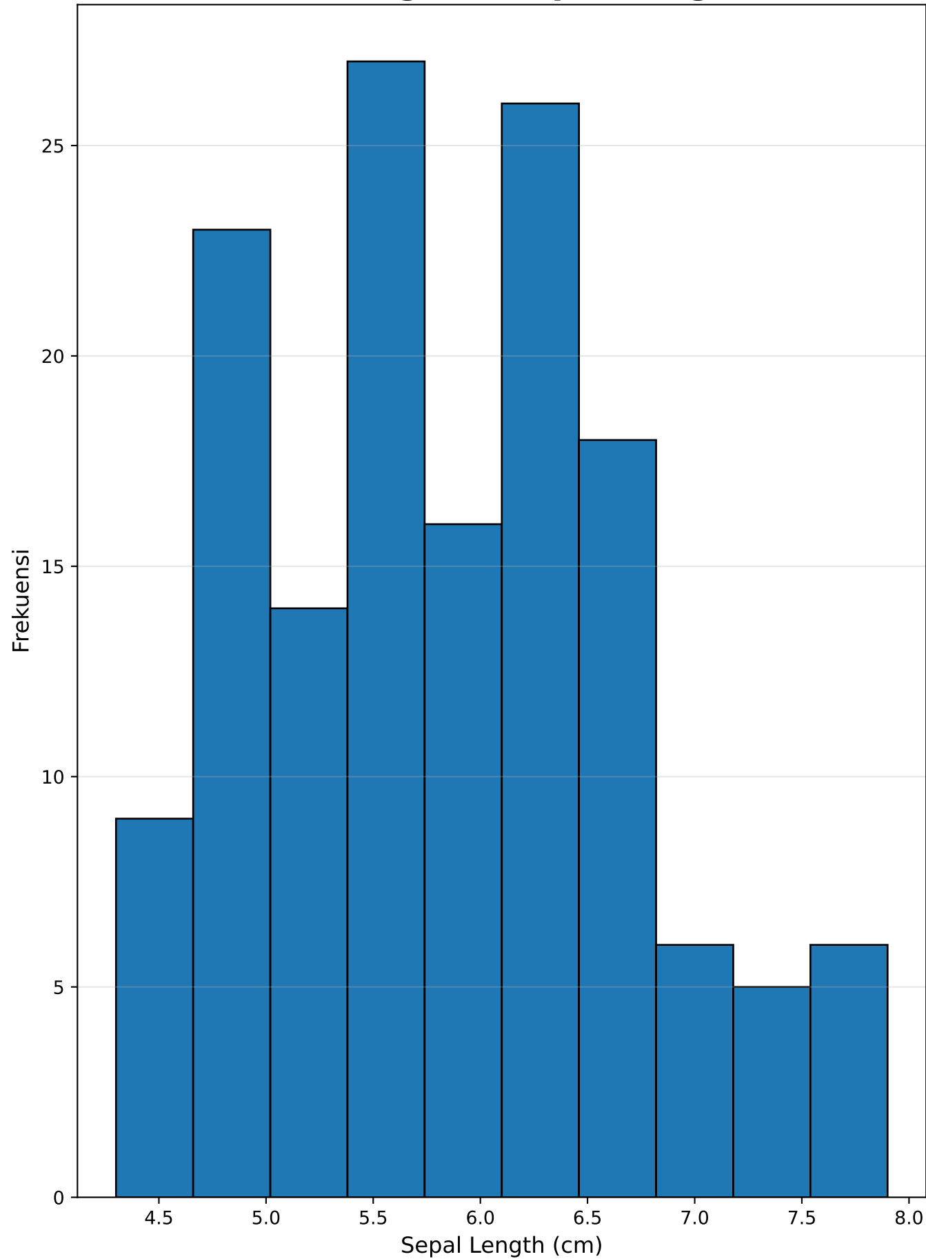
1. Histogram Sepal Length
